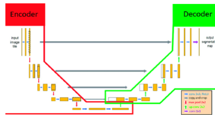
Figure 1. encoder and decoder components on the U-Net Architecture
